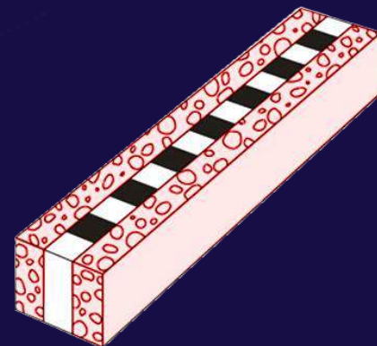
GSG Type With soft foamed silicone isolation layers
